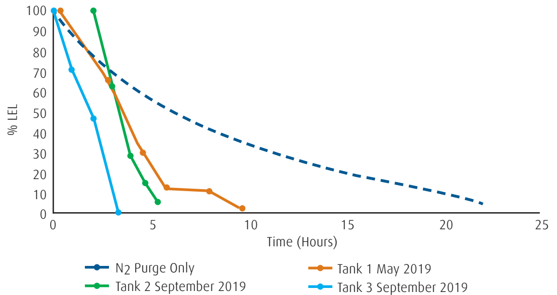
Effect of using the IN2ERT system to LEL free skim tanks
